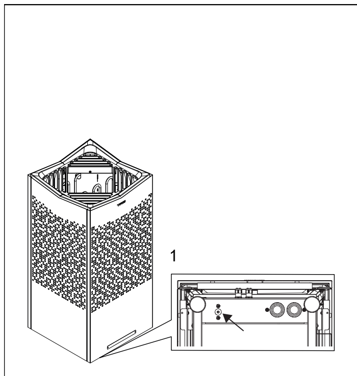
Figure 2: Resetting the temperature cut-out
