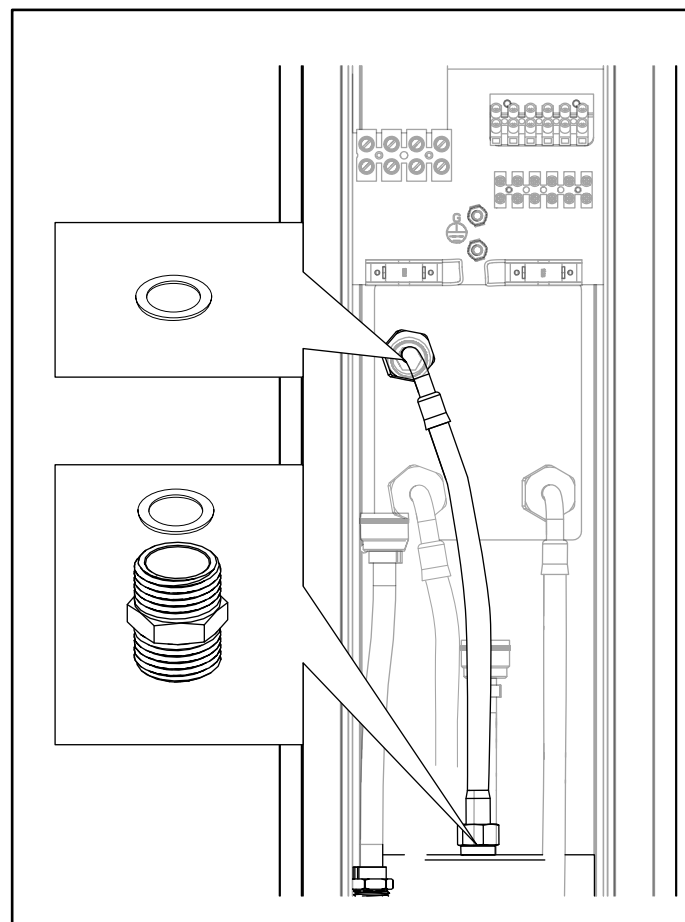
Fig. 5 If an overhead shower is to be installed, remove the end plug and connect the hose. Do not forget the fibre gaskets.
