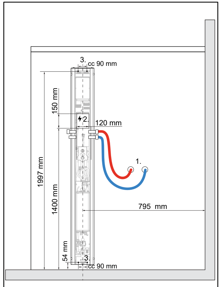
Fig. 4 Connection terminals
