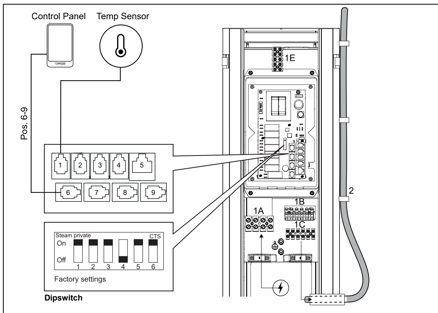
Fig. 5 Schematic diagram of installation, Stella steam generator
