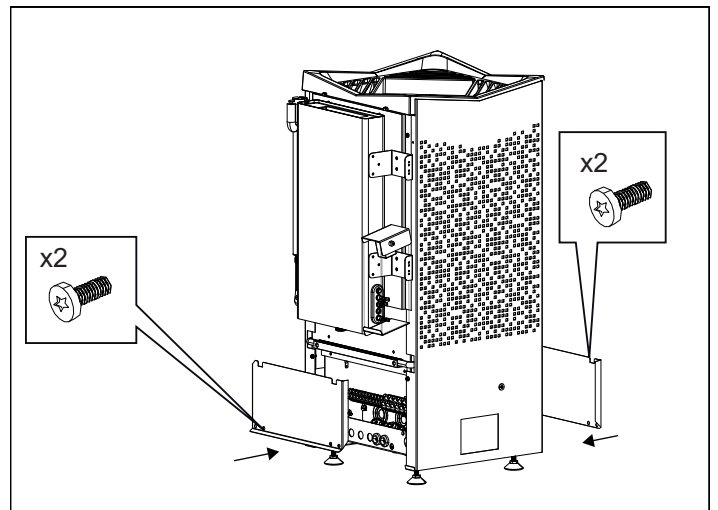
Figure 13: Put back the front and back hatch
